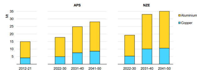
Average annual material needs for transmission and distribution lines in the Announced Pledges Scenario and Net Zero Scenario, 2012-2050
